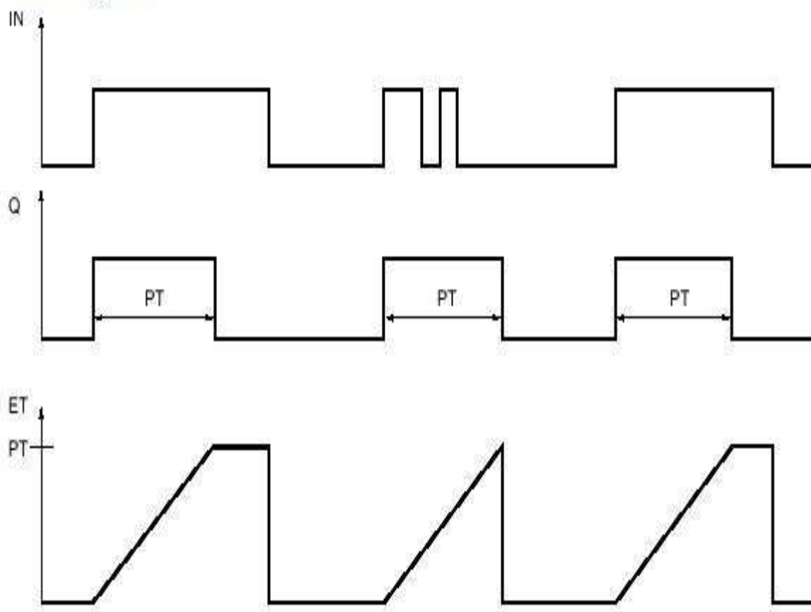
Pulse diagram
