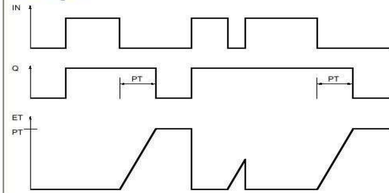
Pulse diagram
